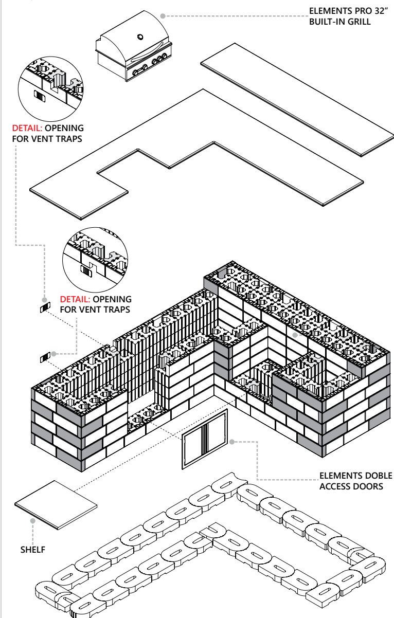
EXPLODED VIEW
