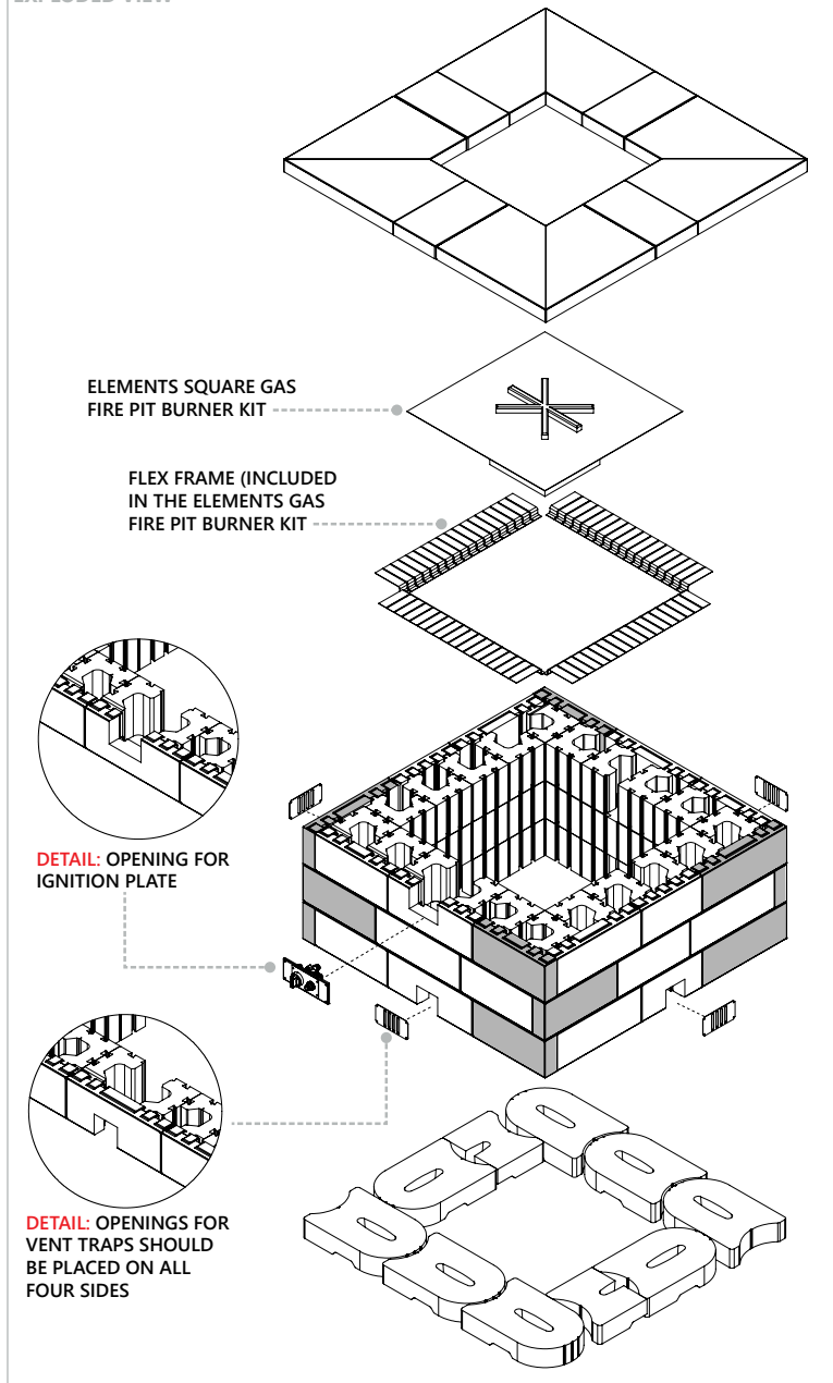
EXPLODED VIEW
