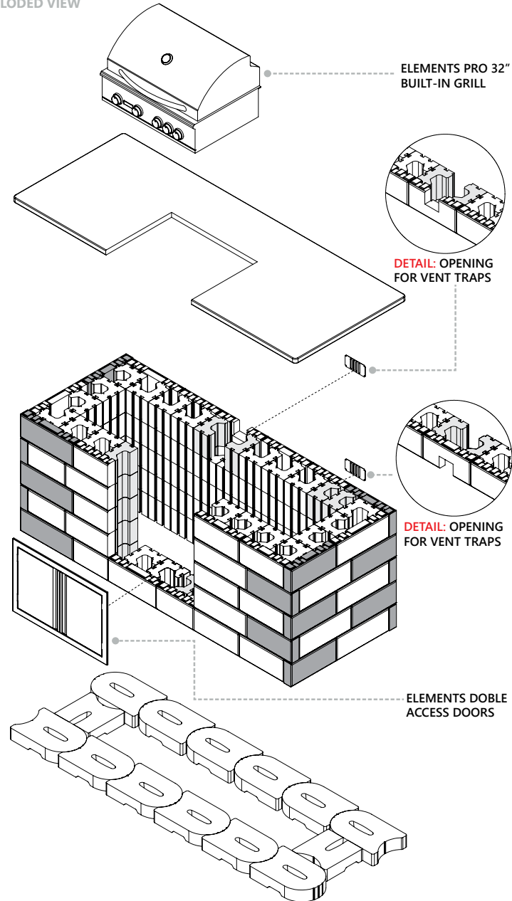
EXPLODED VIEW
