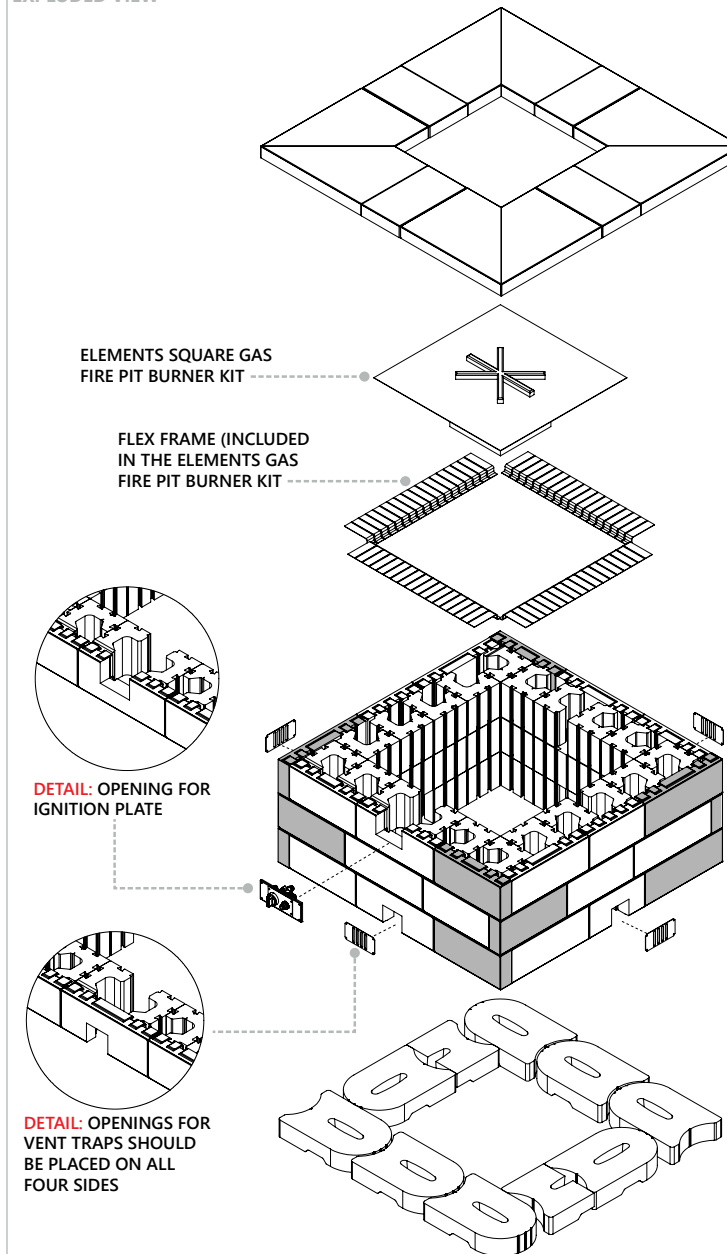
EXPLODED VIEW
