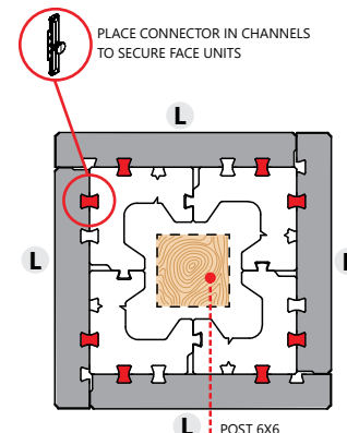
2ND &amp; 4TH COURSE
