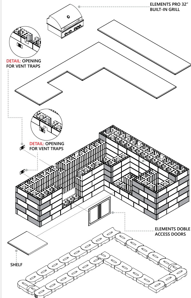
EXPLODED VIEW
