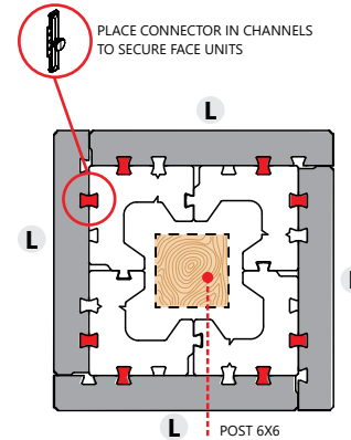
1ST, 3RD &amp; 5TH COURSE
