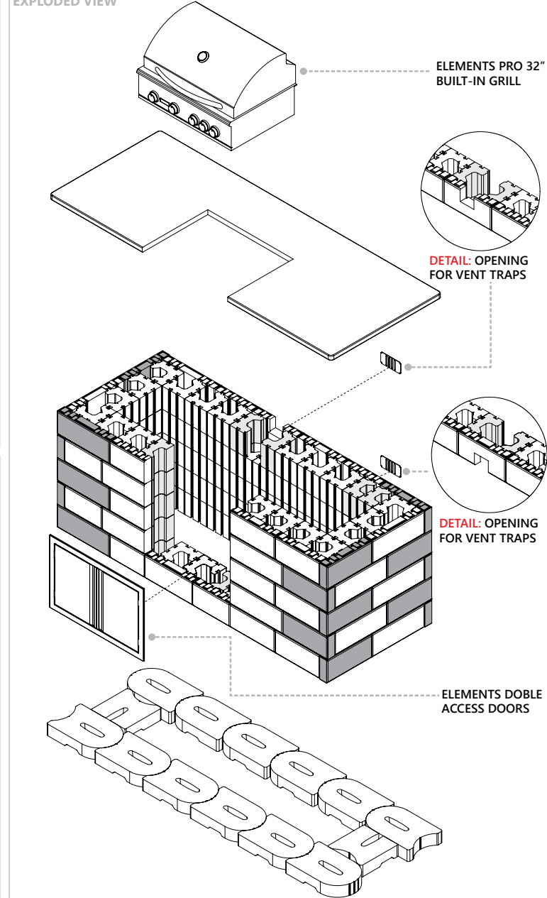
EXPLODED VIEW
