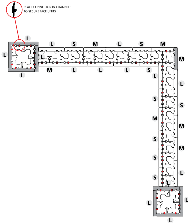
1ST & 3RD COURSE FSW 1ST, 3RD & 5TH COURSE COLUMN
