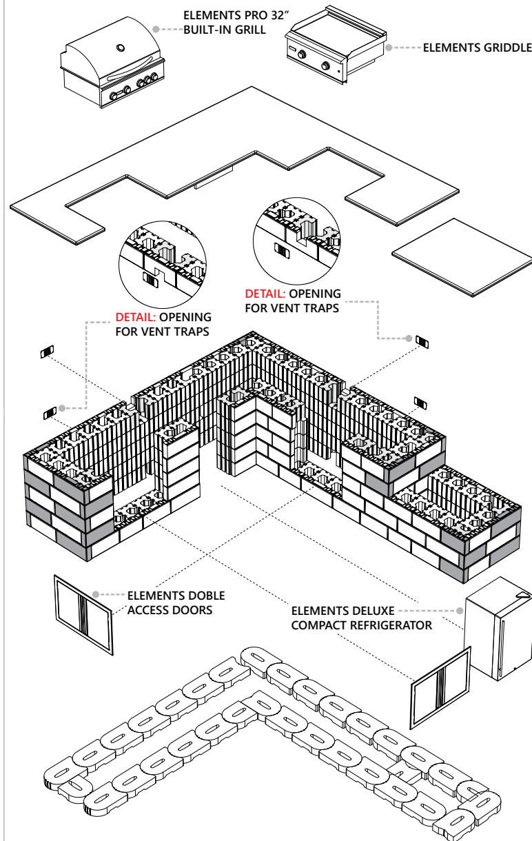
EXPLODED VIEW
