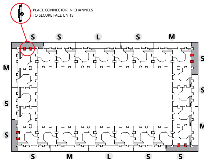
1ST &amp; 3RD COURSE
