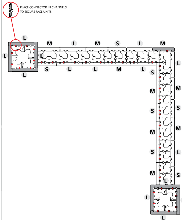
2ND COURSE FSW 2ND, 4TH & 6TH COURSE COLUMN
