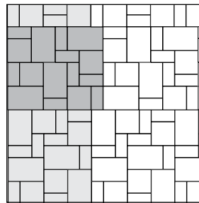
PATTERN 1 64 - 5.7 x 11 32 - 11 x 11 32 - 15 x 17
