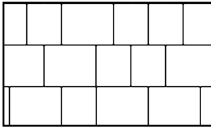
Type 1 & 2 - OFFSET RUNNER BOND Type 1 comprises 60% of total area Type 2 comprises 40% of total area
