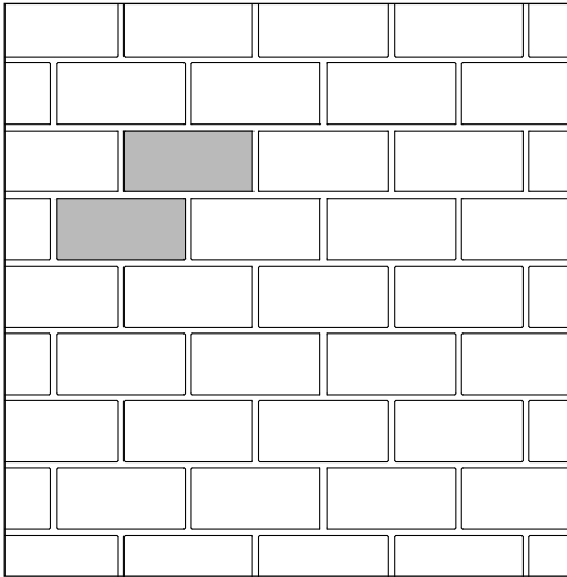
RUNNING BOND
