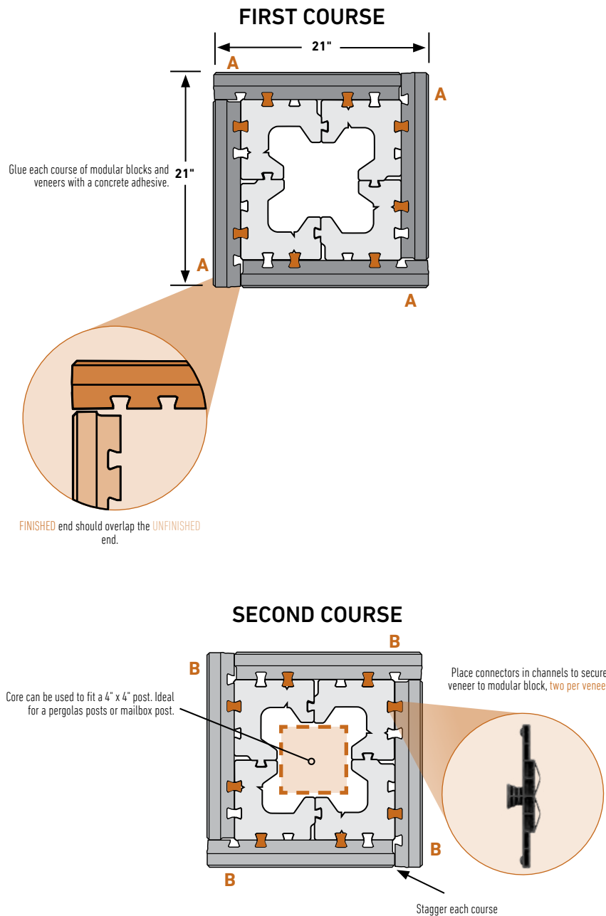
Diagram 24—Connector locations
