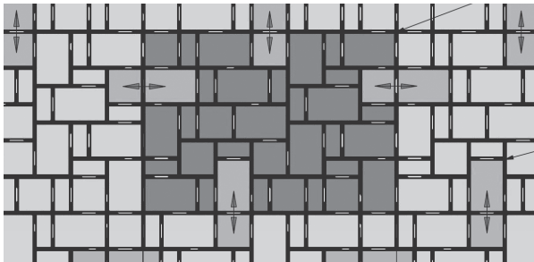
Machine Set Installation Running Bond Pattern
