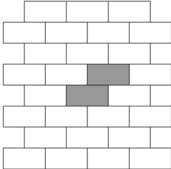
100% LARGE RECTANGLE RUNNING BOND
